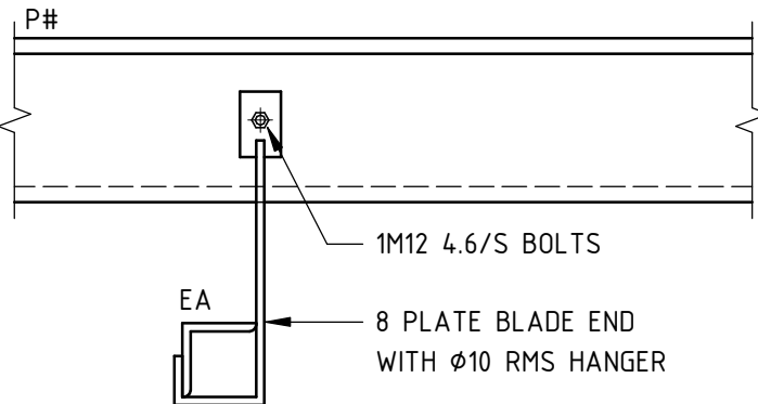
TYPICAL EA SAG ROD DETAIL
