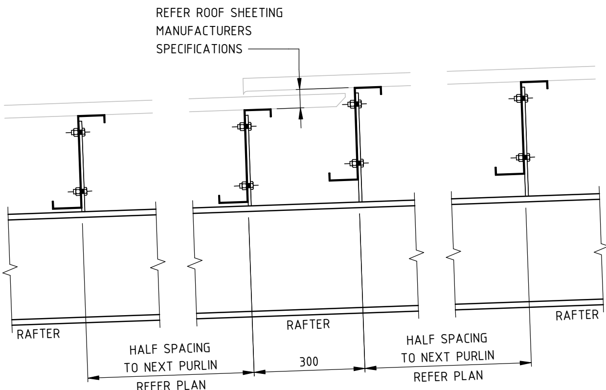
TYPICAL ROOF EXPANSION JOINT DETAIL
