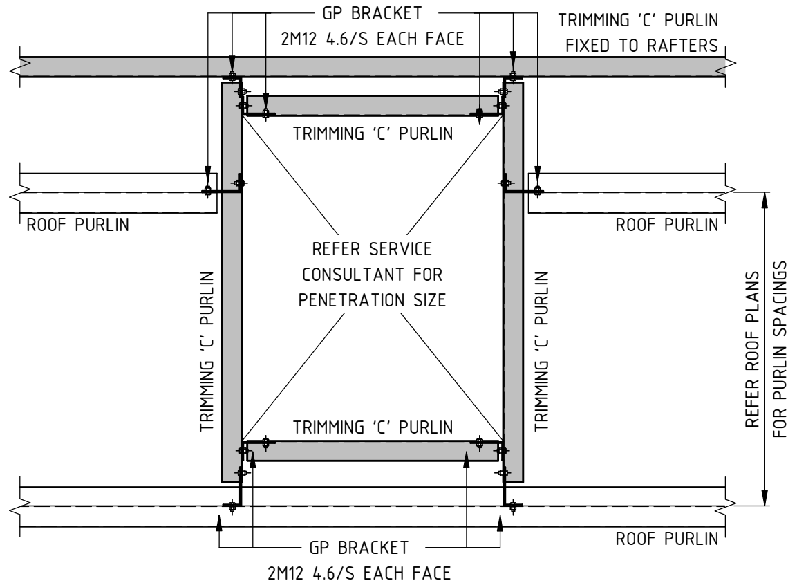
TYPICAL ROOF PENETRATION TRIMMING DETAIL
