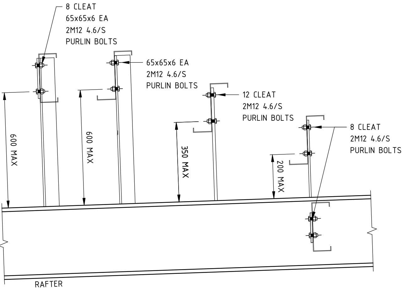
TYPICAL PURLIN AND CEILING JOIST CLEAT DETAIL 100 TO 250 PURLINS, C PURLINS SIMILAR
