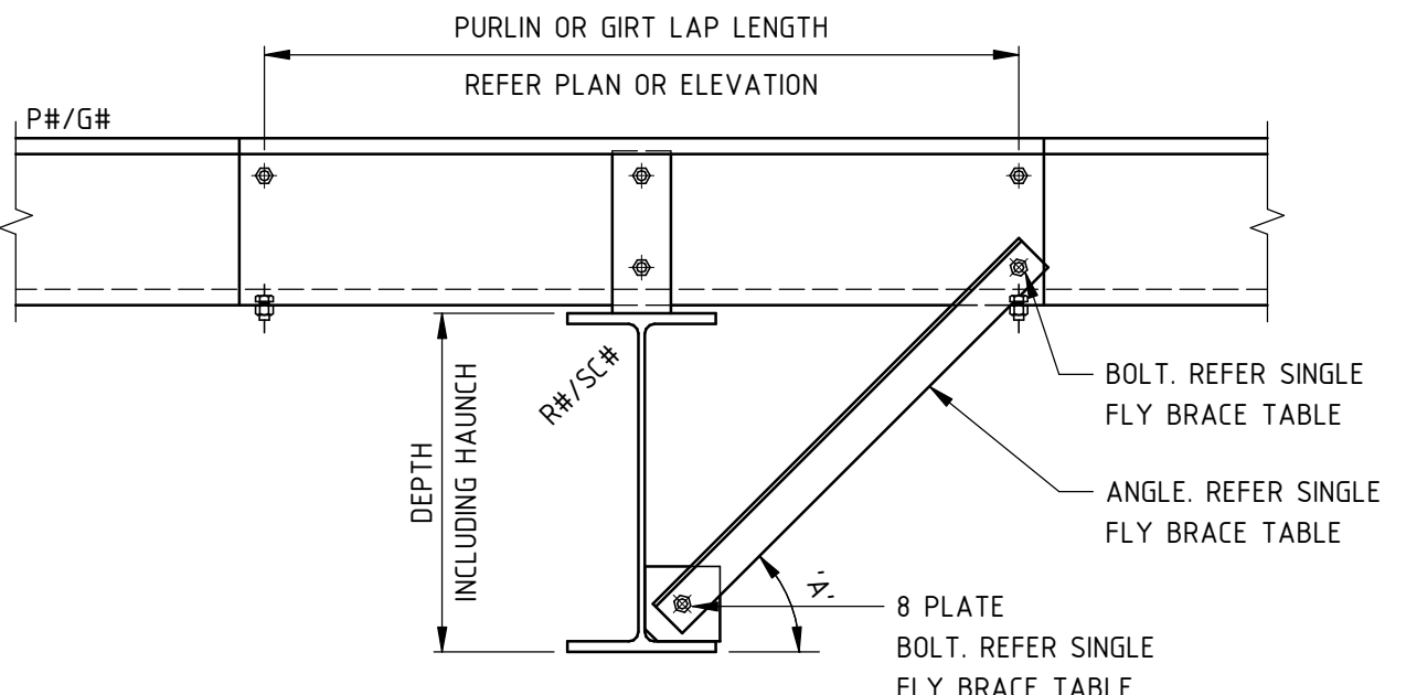
TYPICAL FLY BRACE (FB1) SINGLE SIDE FIXING DETAIL
