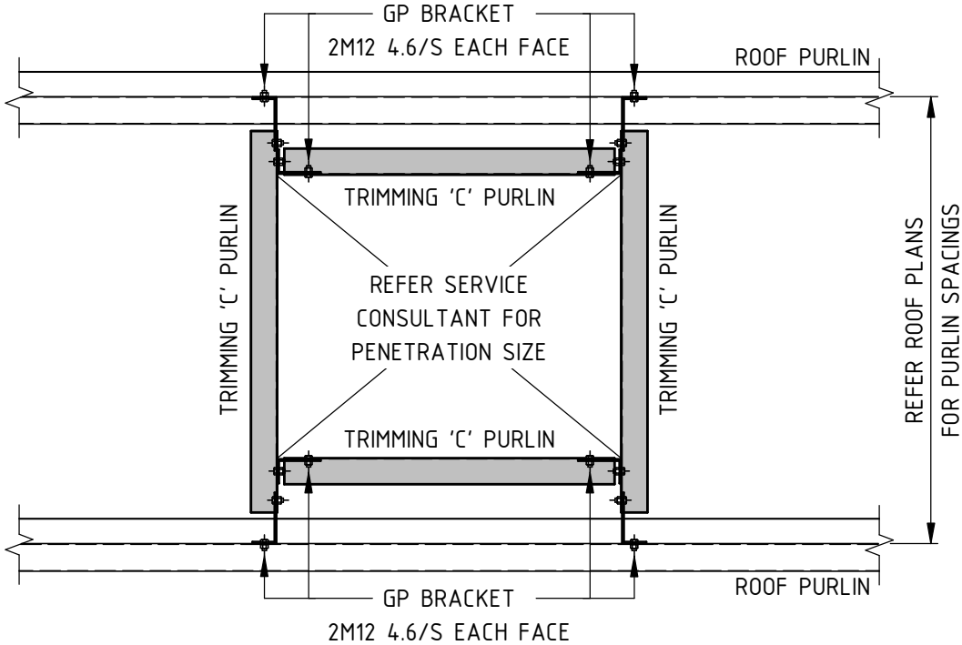
TYPICAL ROOF PENETRATION TRIMMING DETAIL
