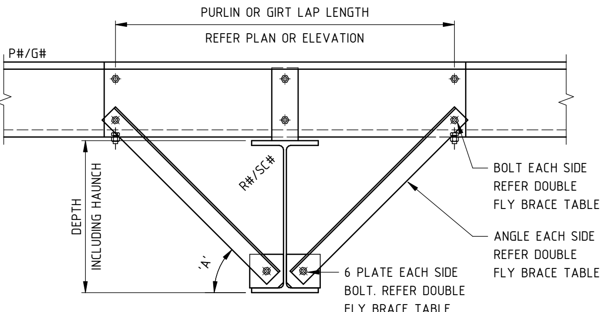
TYPICAL FLY BRACE (FB2) DOUBLE SIDE FIXING DETAIL
