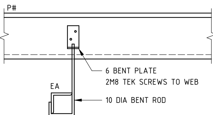
TYPICAL EA SAG ROD DETAIL
